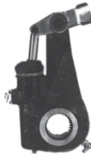
RW-R801041 10-Spline; 1-1/2" 5-1/2" Drilling
